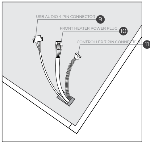
Floor wires
