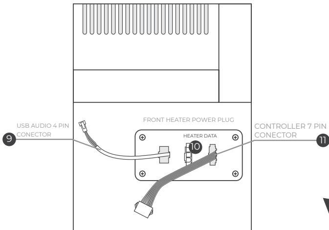
Front panel wires
